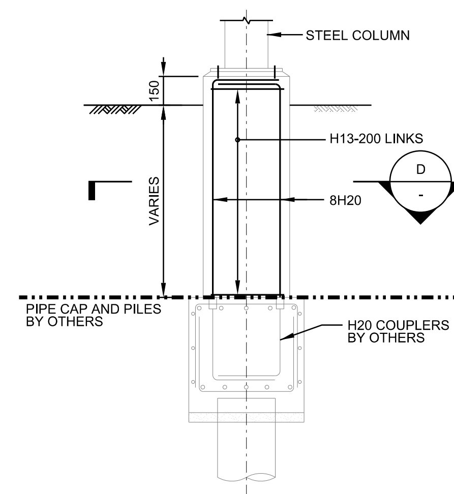
TYPICAL STUMP DETAILS SCALE 1:20
