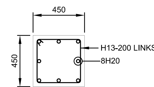
SECTION D - D SCALE 1:20
