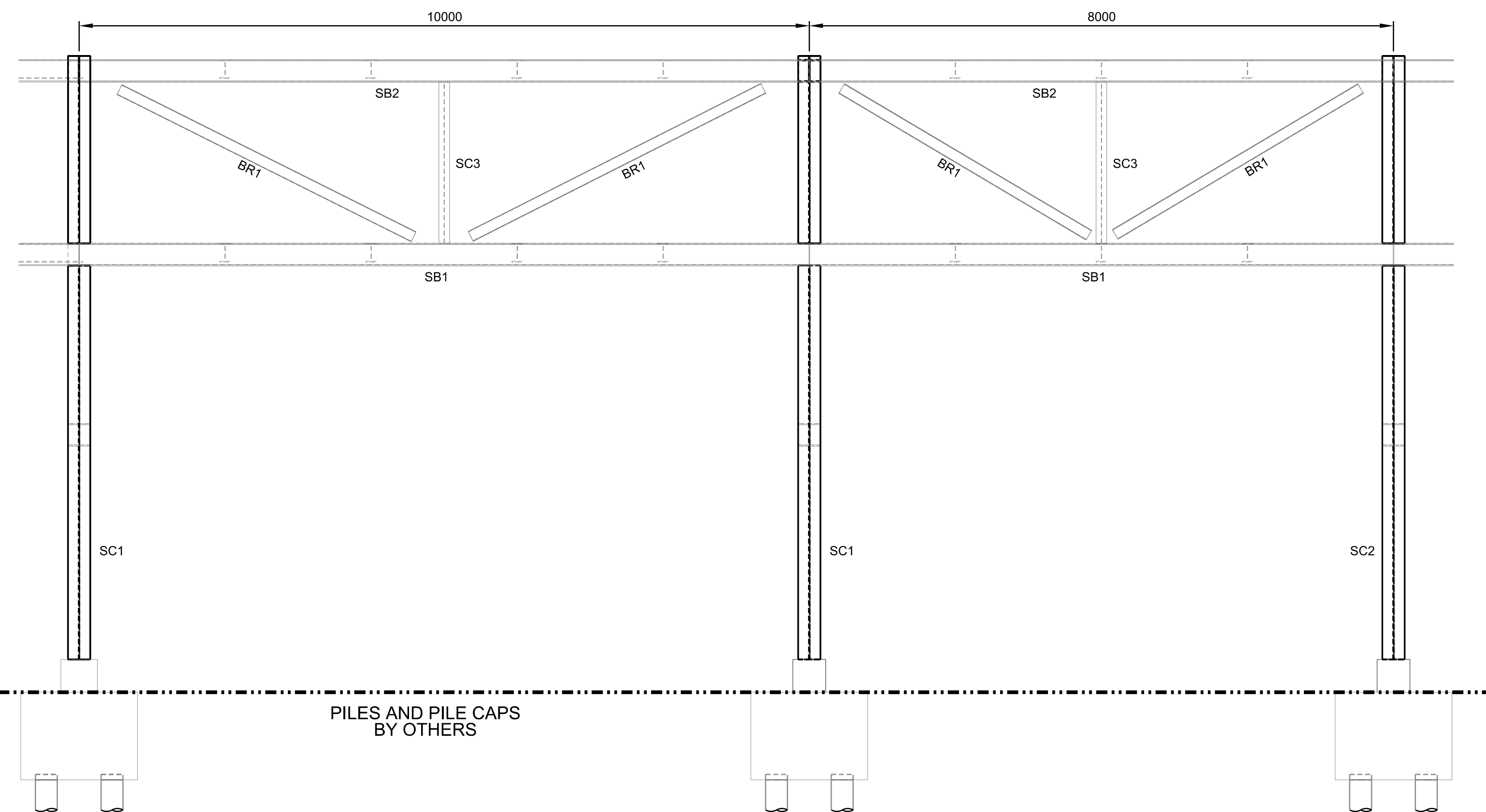
TYPICAL ELEVATION SCALE 1:50
