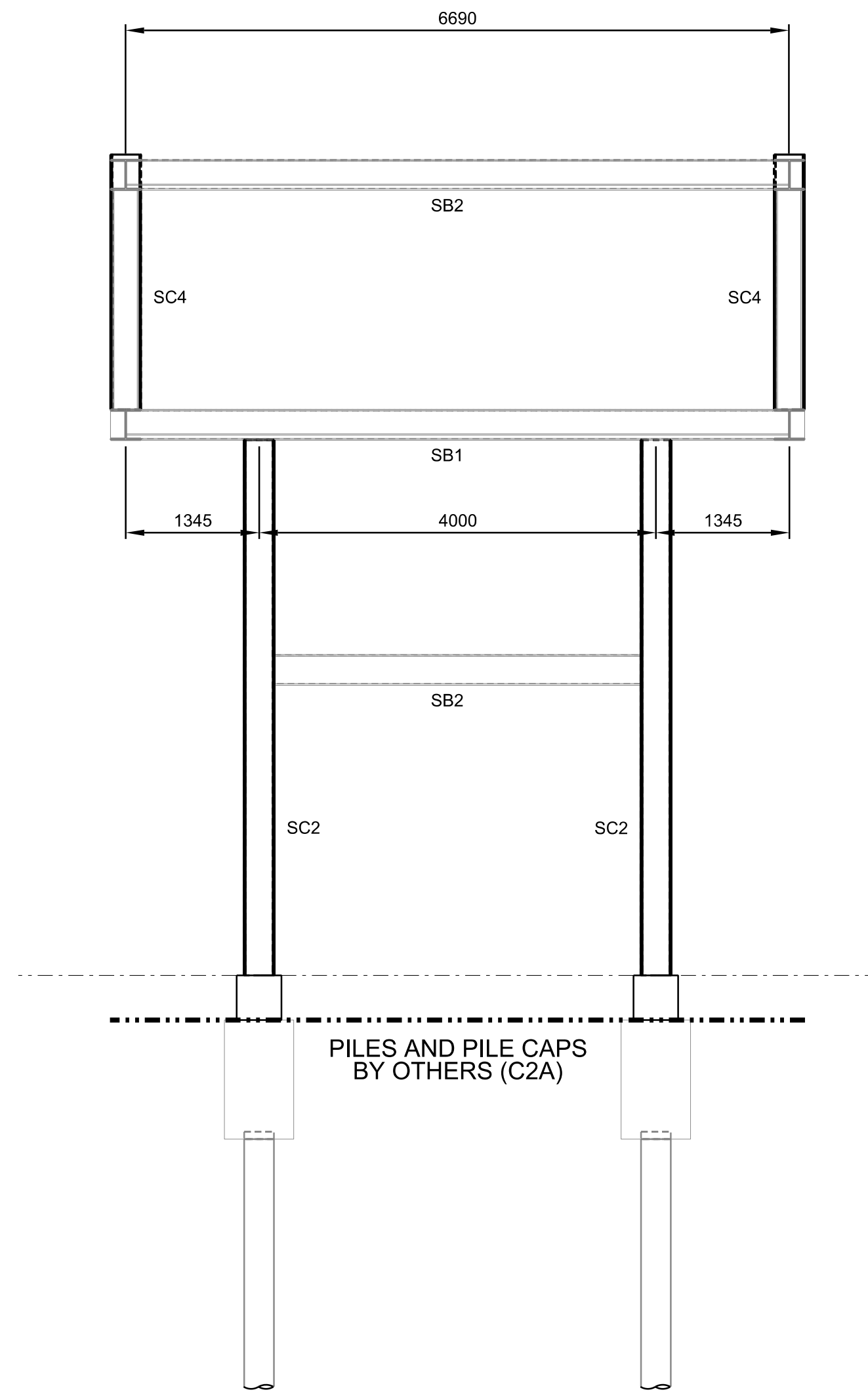
SECTION B - B SCALE 1:50
